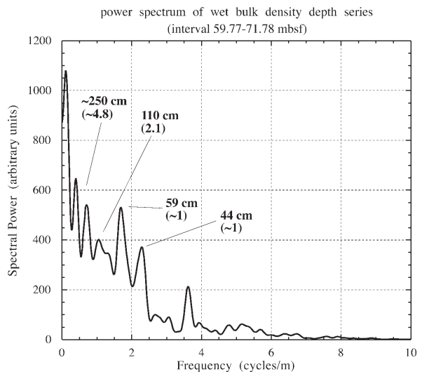
Fig. 5 - Power spectrum of the wet bulk density depth series (interval 59.77-71.78 mbsf). The peaks at 250 cm and at 110 cm match very closely the eccentricity and obliquity ratios. The two peaks centered at 59 cm and 44 cm are interpreted as the two components of the precession cycle (19 and 23 kyr) (see Fig. 4 for explanation).
