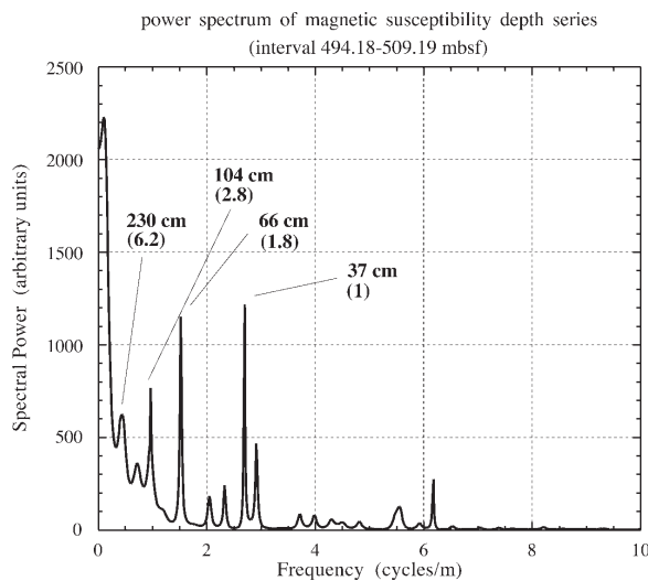
Fig. 9 - Power spectrum of the magnetic susceptibility depth series (interval 494.18-509.19 mbsf). Assuming that the line at 37 cm refers to the precession cycle, the periodicity at 66 cm corresponds to the obliquity, while the group of lines at 104 and 230 cm gives an intermediate ratio for the eccentricity cycles (see Fig. 4 for explanation).
