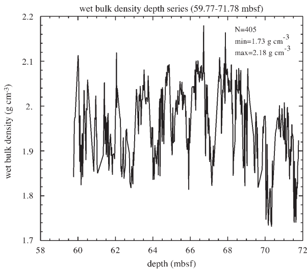
Fig. 3 - Wet bulk density depth series (interval 59.77-71.78 mbsf).
