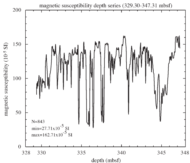
Fig. 6 - Magnetic susceptibility depth series (interval 329.30-347.31 mbsf).
