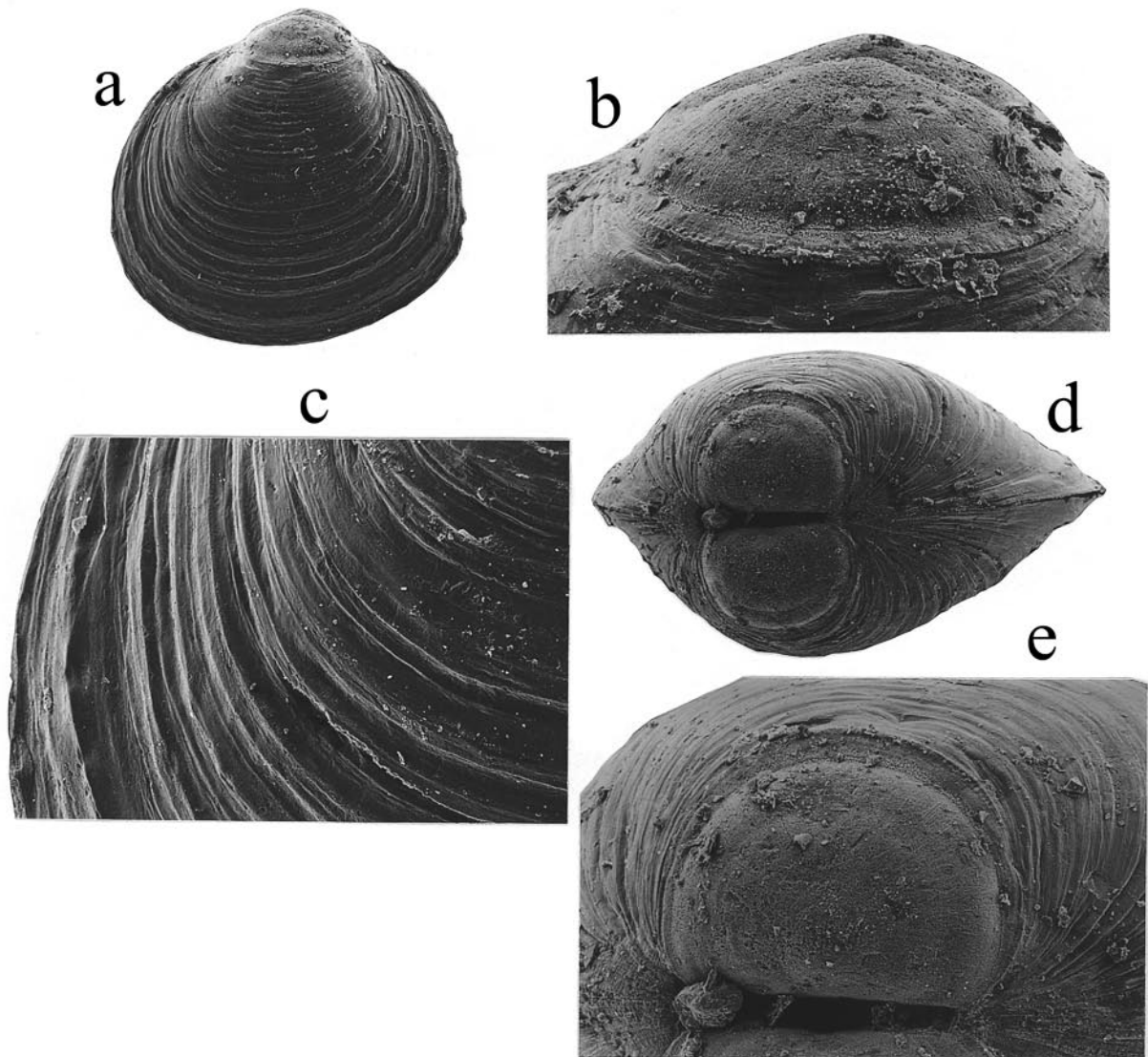
Fig. 4 - ?Phylobriidae, unidentified, (Late Oligocene, LSU 9.4, 227.39 mbsf), complete articulated specimen, width 1.4 mm: (a) right valve, enlarged x 40; (b) lateral view of prodissoconch of right valve, enlarged x 160; (c) sculpture of posterior area of right valve, enlarged x 160; (d) dorsal view of whole shell, enlarged x 60; (e) dorsal view of right valve prodissoconch, enlarged x 125. SEM photographs.
