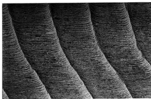
Fig. 7 - ? Adamussium n.sp.; (a) SEM photograph showing highly oblique view of commarginal frills and antimarginal microsculpture of ? Adamussium n. sp. (Early Miocene, LSU 5.1, 71.42 mbsf; dorsal is to the right); (b) SEM photograph showing highly oblique view of commarginal frills and antimarginal microsculpture on a right valve of Adamussium colbecki from Explorers Cove, McMurdo Sound, Ross Sea (specimen courtesy of Paul Arthur Berkman); dorsal is to the right. Note that growth increments are much wider than in the Oligocene fossil.
