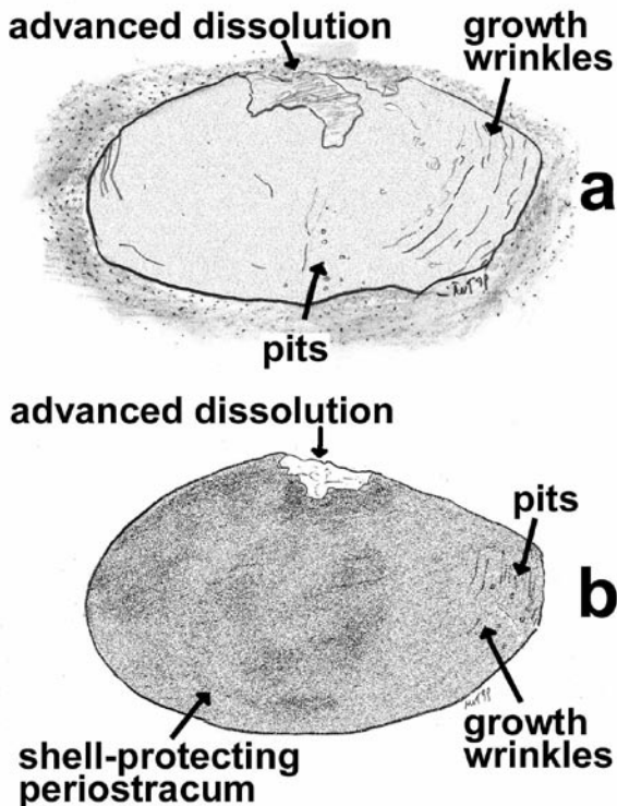
Fig. 5 - Comparison of shell features on external valve of (a) Yoldia ( Aequiyoldia ) sp. (Late Oligocene, LSU 9.7, 260.83 mbsf) and (b) Yoldia ( Aequiyoldia ) eightisi (Recent, McMurdo Sound, 30 metres); camera lucida hand drawing (M.T.) elaborated by Stefano Parisini.
