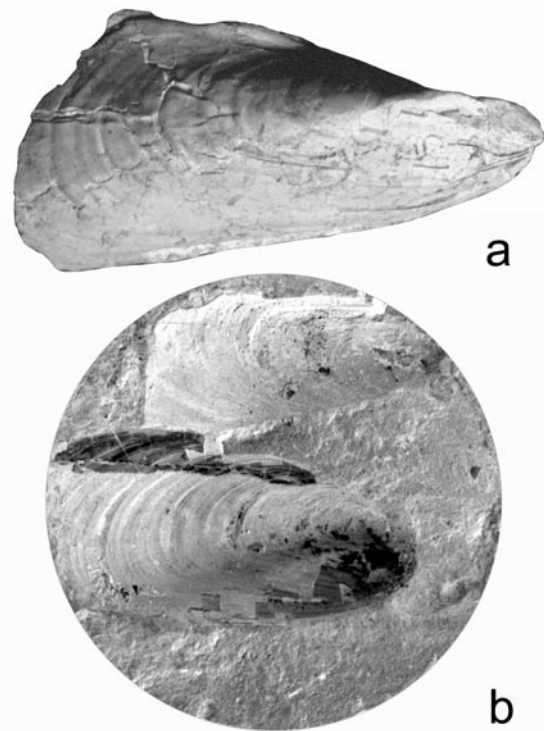
Fig. 6 - ? Modiolus sp. (Early Oligocene, LSU 13.1); (a) internal mould of articulated shell, 449.64 mbsf; (b) complete articulated shell with valves open (447.43 mbsf: printed as a negative to enhance visibility of ornamentation).
