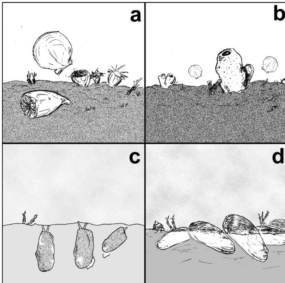
Fig. 8 - Cartoons depicting artistic reconstructions of Roberts Ridge sea-bottom at selected time-slices: (a): Early Miocene, LSU 3.1. at c. 36 mbsf: middle-outer shelf environment dominated by suspension feeders, including solitary corals, large pectinids ( Adamussium n. sp.) and serpulid polychaetes (water depth 40-100 m?); (b), Early Miocene, LSU 8.1 at c. 117 mbsf: middle-outer shelf environment dominated by epifaunal (sponges and pectinids) and semi-infaunal suspension feeders (water depth 40-80 m?) (c) Late Oligocene, LSU 9.7 at c. 165 mbsf: fine-grained, relatively shallow (20-40 m?) shelf environment dominated by deposit ( Yoldia and other protobranchs) and suspension (serpulid polychaetes) feeders in turbid waters; (d) Early Oligocene, LSU 13.1 at c. 464 mbsf: deep-shelf/upper-slope fine-grained, H 2 S-enriched environment dominated by dense aggregates of semi-infaunal modiolid bivalves, with associated gastropods and serpulid polychaetes; (hand drawings by M.T., computer-elaborated by Stefano Parisini).
