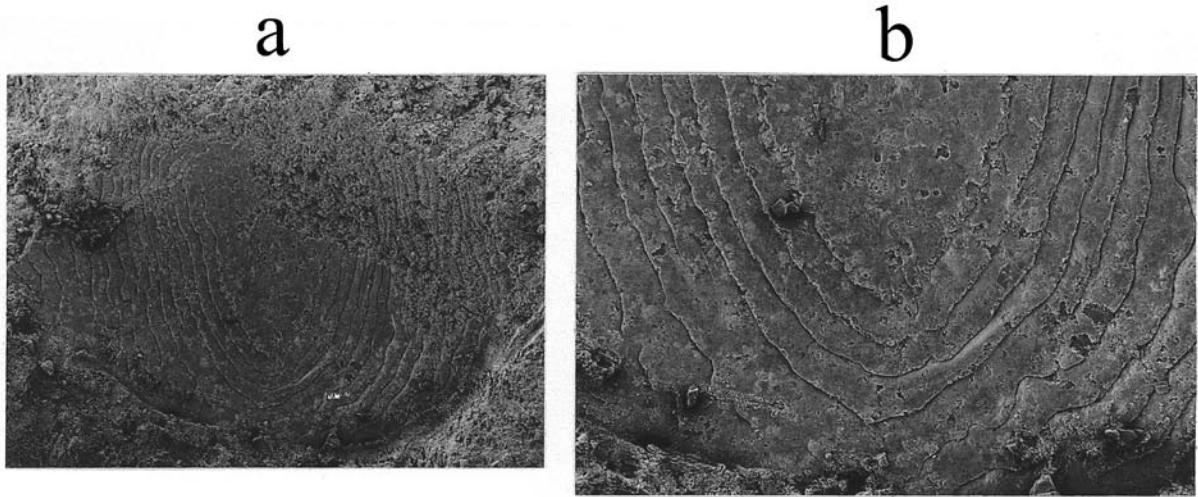
Fig. 3 - Unidentified fish scale, (Late Oligocene, LSU 8.4, 166.64 mbsf): natural mould of incomplete scale, width 4.2 mm: (a) general view, enlarged x 17; (b) detail, enlarged x 40. SEM photographs.
