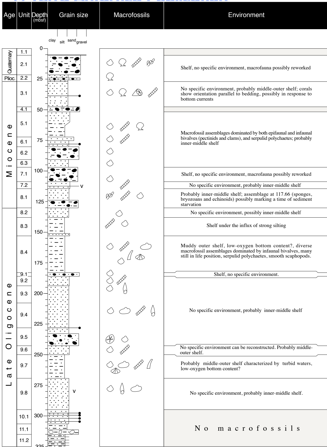
Fig. 1 - Lithostratigraphical summary of CRP-2/2A drill core showing position and composition of the major macrofossil assemblages and their palaeoenvironmental significance (slightly modified from Cape Roberts Science Team, 1999).
