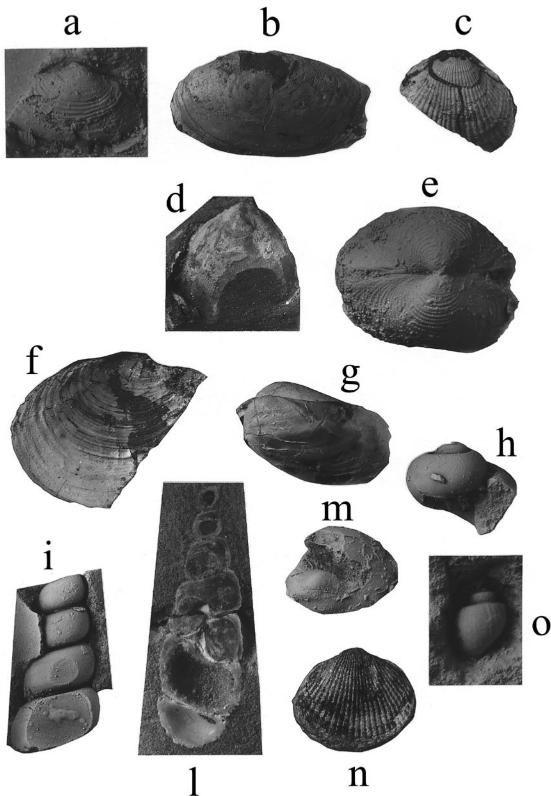
Fig. 2 - Early Miocene and Oligocene macrofossils from CRP-2/2A drill core: (a) ?Neilo sp. (Late Oligocene, LSU 9.7, 257.60 mbsf); incomplete right valve, length 8.5 mm); (b) Yoldia (Aequiyoldia) sp. (Late Oligocene, LSU 9.7, 260.83 mbsf); slightly incomplete left valve, length 21 mm. (c) Cyclocardia sp.; (Late Oligocene, LSU 9.3, 195.36 mbsf), incomplete articulated shell, length 10.7 mm. (d) Cardiidae? , (Early Oligocene, LSU 13.1, 446.59 mbsf), incomplete decorticated valve, height 13.2 mm. (e) Veneroidean bivalve, (Late Oligocene, LSU 9.4, 224.41 mbsf), incomplete articulated shell, width 9.9 mm. (f) Periploma sp. (Early Oligocene, LSU 13.1, 443.91 mbsf), incomplete right valve, length 21 mm. (g) Hiatella sp. (Early Oligocene, LSU 13.1, 450.68 mbsf), slightly oblique dorso-lateral view of incomplete internal mould of articulated shell, length 16 mm. (h) Trochoidean? gastropod, (Early Oligocene, LSU 13.1, 448.58 mbsf), apertural view of internal mould, diameter 9.5 mm. (i) Turritellidae, indet., (Late Oligocene, LSU 9.8, 285.12 mbsf), incomplete internal mould, height 24 mm. (l) Turritellidae, indet., (Late Oligocene, LSU 9.4, 226.85 mbsf), formerly complete shell sectioned by drill, height 22 mm. (m) ?Crepidula sp., (Early Oligocene, LSU 13.1, 446.59 mbsf), oblique latero-dorsal view of incomplete internal mould, length 10 mm. (n) Rhynchonellid? brachiopod, (Late Oligocene, LSU 9.7, 262.02 mbsf), dorsal view of slightly incomplete dorsal valve, width 11 mm. (o) Neogastropod, undetermined (Cancellariidae?), (Early Oligocene, LSU 13.1, 446.59 mbsf), dorsal view of internal mould, height 4.5 mm.
