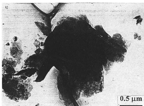
Fig. 5 - TEM images showing: a) at core level 64.58 mbsf, a hairy Fe-rich smectite particle; b) at core level 229.19 mbsf, a hairy Fe-Al smectite particle; c) at core level 252.07 mbsf, a hairy Fe-rich smectite particle; d) at core level 309.74 mbsf, a hairy Fe-Al smectite particle; e) at core level 604.5 mbsf, a hairy smectite developed on a flaky one.
