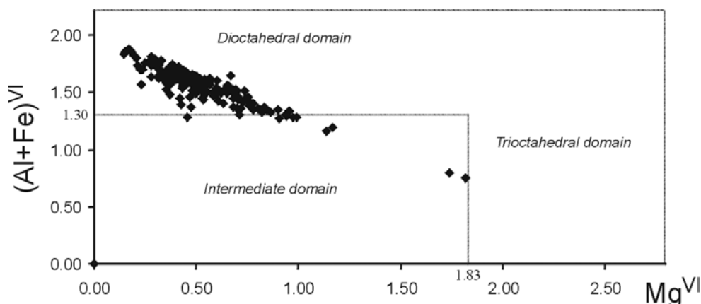
Fig. 1 - Octahedral composition of individual particles of smectites: (Al+Fe)^{VI} vs. Mg^{VI} . The compositional fields of dioctahedral, intermediate and trioctahedral domains are reported.
