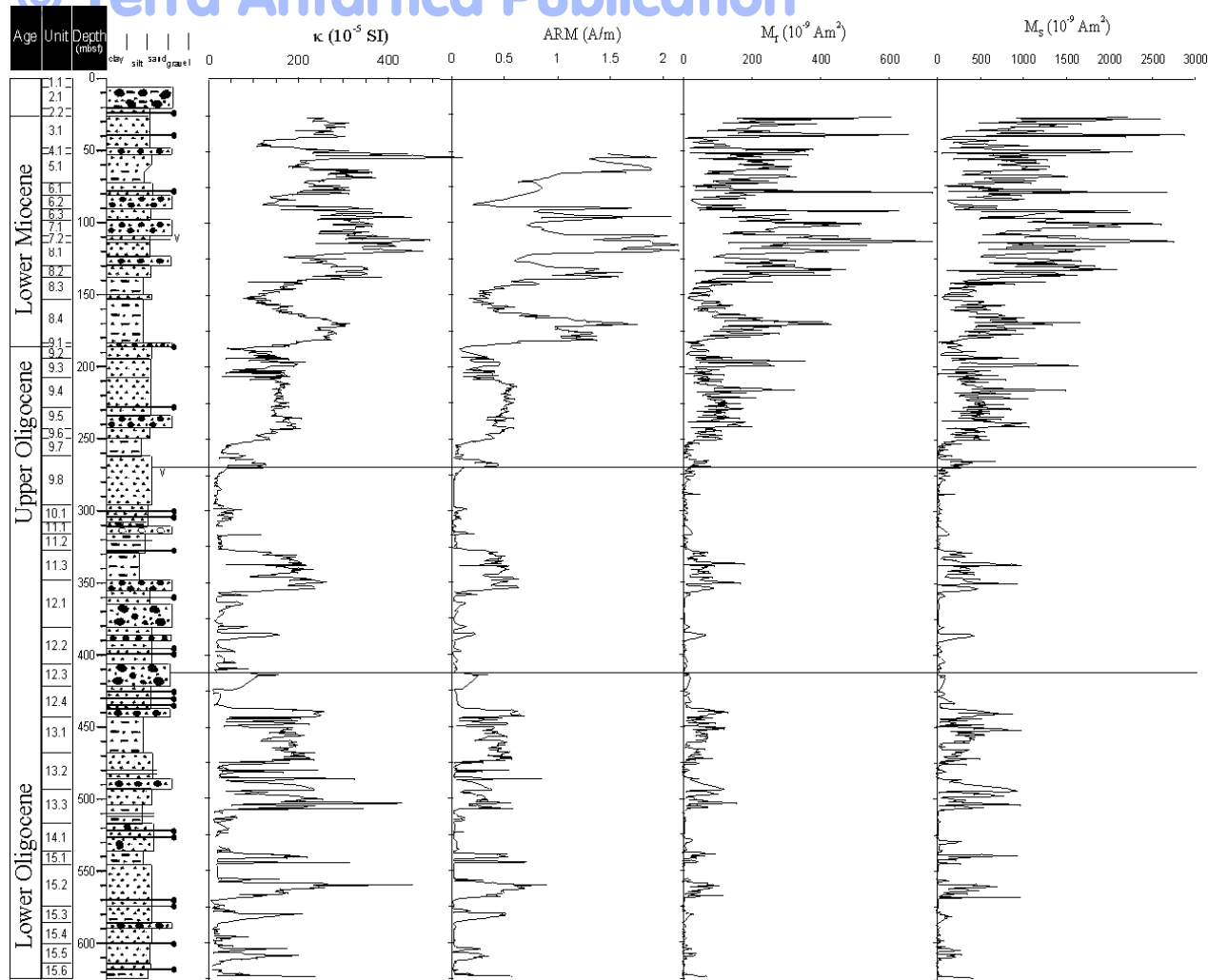
Fig. 1 – Down-core variation of ferrimagnetic concentration-dependent parameters ( \kappa , ARM, M_r and M_s ) in CRP-2/2A. The lines at 270 and 413 mbsf indicate the boundaries between intervals with different magnetic properties (see discussion in text, Fig. 2 & Tab. 1).
