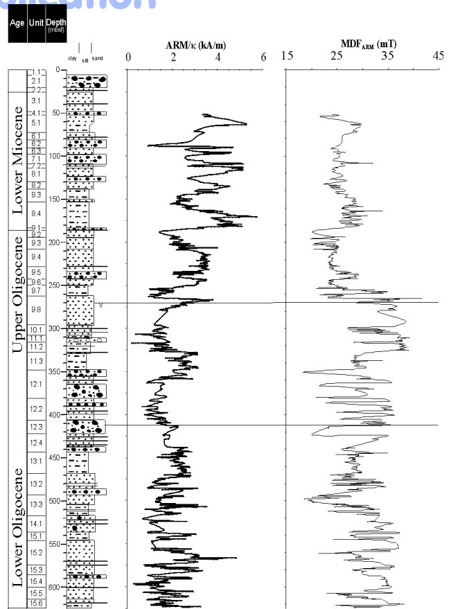
Fig. 5 – Down-core variations of ARM/ \kappa and MDF_{ARM} for CRP-2/2A. The lines at 270 and 413 mbsf indicate the boundaries between intervals with different magnetic properties.
