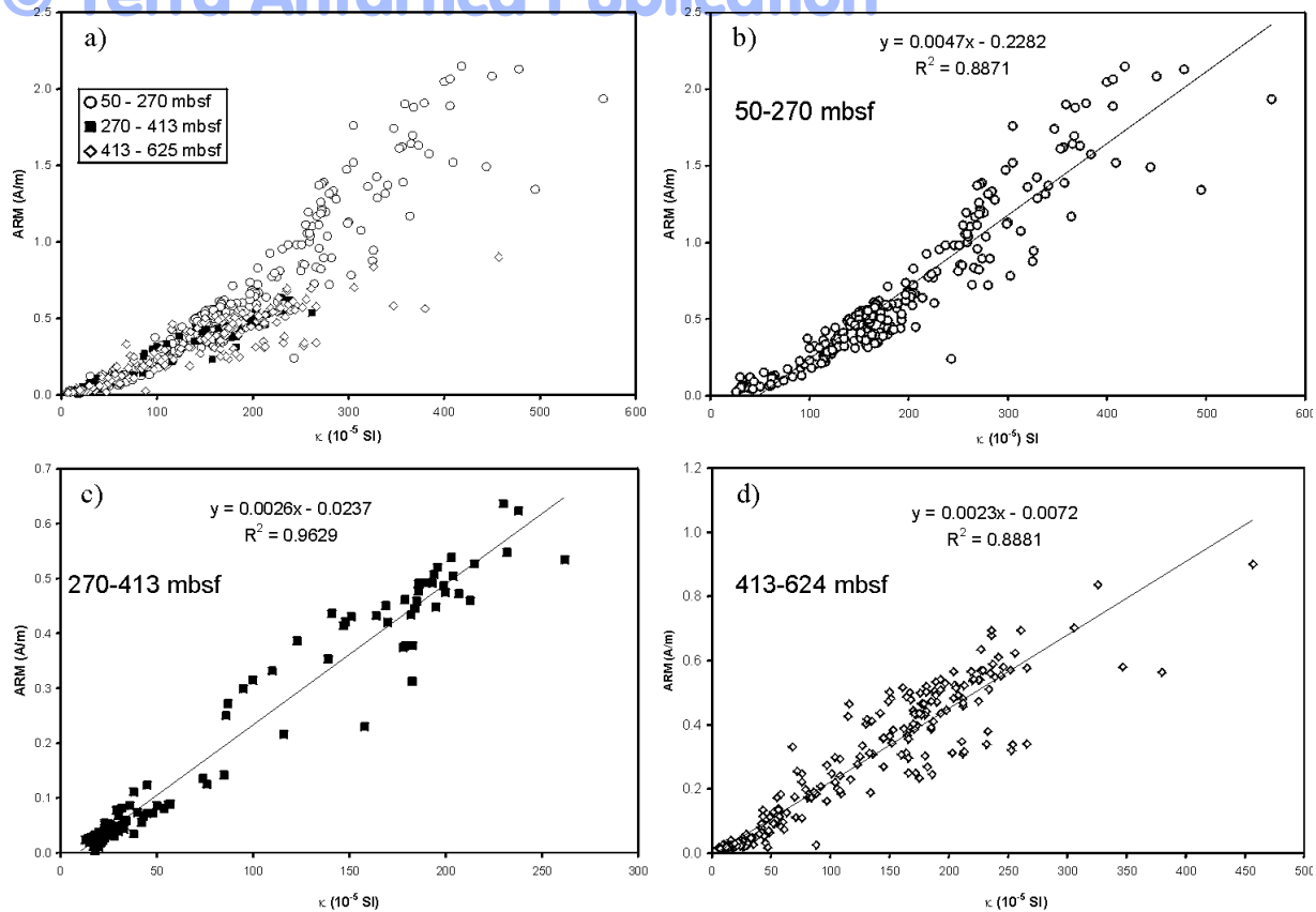
Fig. 6 – Plots of ARM versus \kappa for: a) all data from CRP-2/2A, b) the interval between 50 and 270 mbsf, c) the interval between 270 and 413 mbsf, and d) the interval between 413 and 624 mbsf (see discussion in text). Note that the scales on the axes and hence the slopes of the lines are different in each plot.
