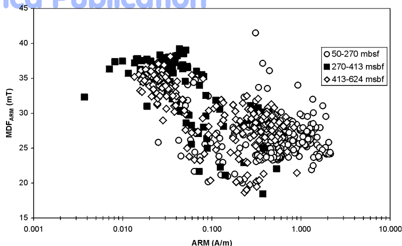
Fig. 7—Plots of MDF_{ARM} versus ARM for all data from CRP-2/2A. Two clusters of samples can be distinguished: one with low ARM intensities and relatively high MDF_{ARM} values corresponds to hematite-enriched samples; the other with high ARM intensities and low MDF_{ARM} values corresponds to magnetite-enriched samples. The points scattered between these clusters represent samples with a mixture of magnetite and hematite.
