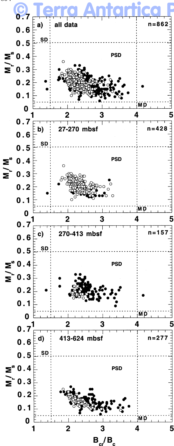
Fig. 4 – Plots of M_r/M_s versus B_{cr}/B_c for: a) all data from CRP-2/2A, b) the interval between 27 and 270 mbsf, c) the interval between 270 and 413 mbsf, and d) the interval between 413 and 624 mbsf. Open symbols correspond to points with high magnetic mineral concentration; closed symbols correspond to points with low magnetic mineral concentration. The fields marked for SD = single-domain, PSD = pseudo-single-domain, and MD = multi-domain, correspond to the ranges of values expected for crushed (titano)magnetite grains (Day et al., 1977).
