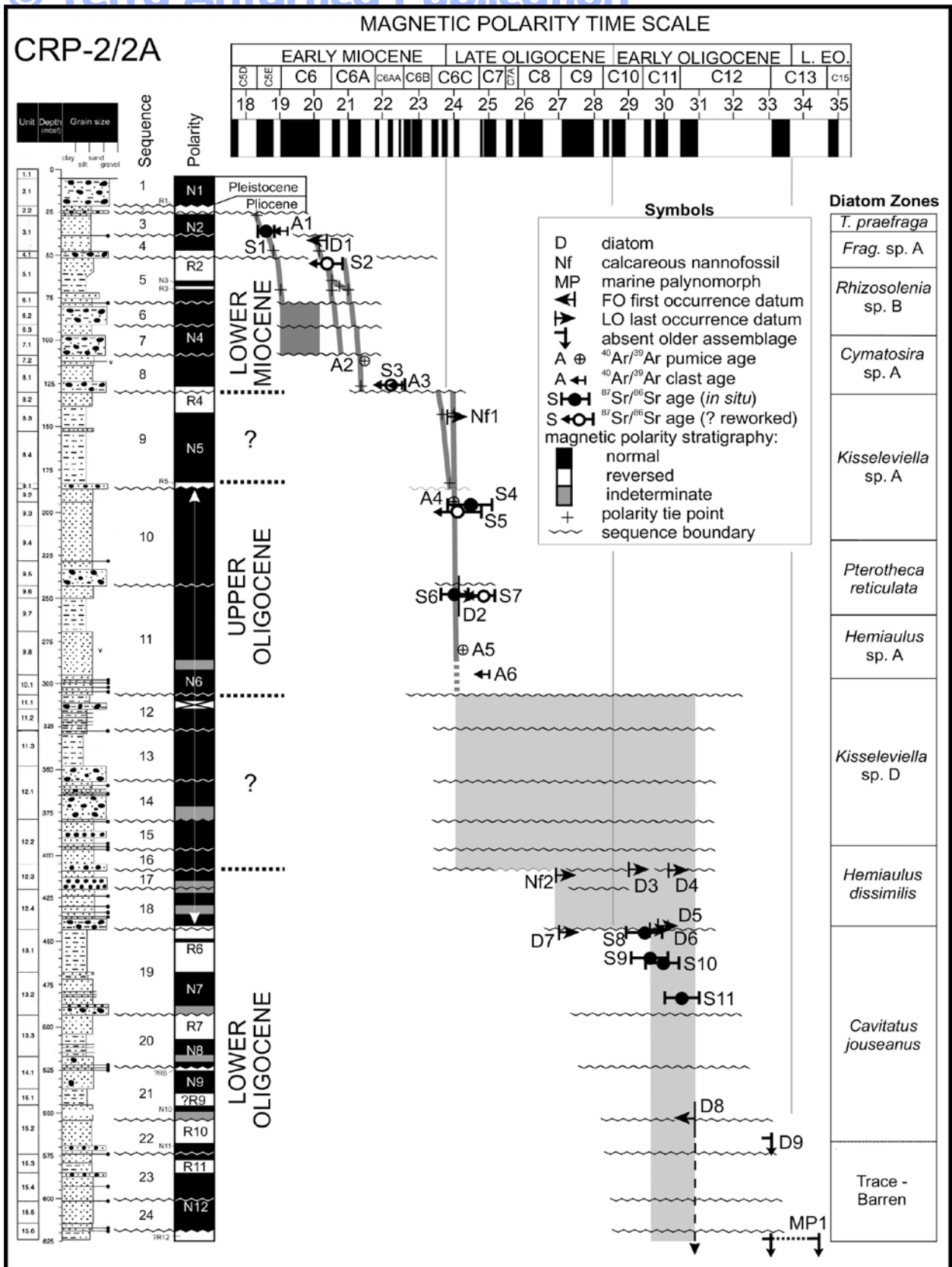
Fig. 1 - Age model for the CRP-2/2A drillcore. The age model is based on biostratigraphy, ^{40}\text{Ar}/^{39}\text{Ar} ages of volcanic material, ^{87}\text{Sr}/^{86}\text{Sr} analyses of mollusc shells and magnetostratigraphy. The stratigraphic column, with lithological units and sequence stratigraphic interpretations, is from Cape Roberts Science Team (1999). Datum events, with alphanumeric indicators that are used to constrain the correlation, are listed in Table 1. The length of vertical bars on biostratigraphic datums indicates the range of error from the respective sampling interval on which the datums are defined. Undulating lines represent sequence bounding unconformities where time loss is predicted. Above 306.65 mbsf, possible correlations to the MPTS are indicated by dark grey lines. Between 306.65 and 624.15 mbsf, no unique correlation to the MPTS is possible. Above 306.65 mbsf, correlation lines represent average sediment accumulation rates. Actual sedimentation rates may be higher. Palaeomagnetic polarity was not determined for the intraformational breccia between c. 311 and 315 mbsf. Light grey shading within the main diagram indicates the range of possible age-depth correlations based on biostratigraphic data.
