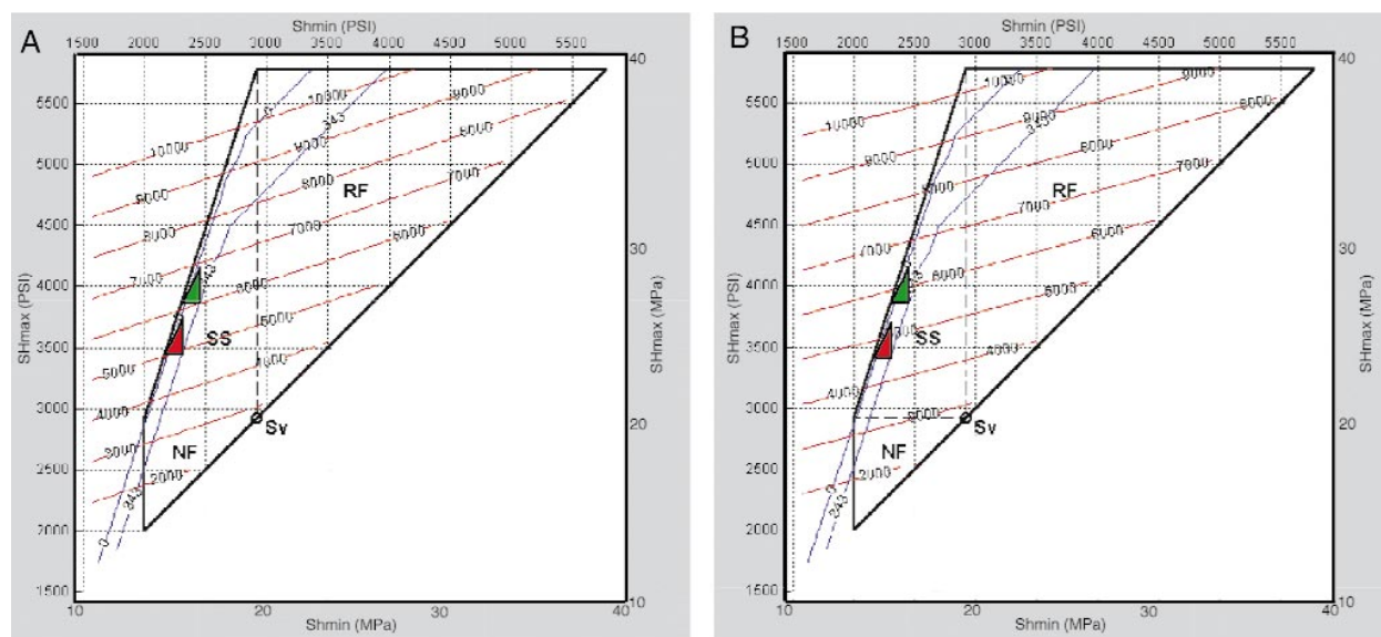
Fig. 3 - Constraints on stress magnitudes at a depth of approximately 1030 mbsl. The frictional strength polygon is black, red contours are conditions for breakouts (in psi), and blue contours are conditions for wall fractures (in psi). A: conditions that would cause breakouts to begin to form ( wBO=0 ) while no circulation is occurring. The blue lines indicate bounding conditions to generate tensile cracks while pumping (excess pressure of 343 psi, or 2.4 MPa) and to avoid tensile cracks while not pumping (0 excess pressure). For a least stress of 2400 \pm 100 psi (16.6 MPa), the shaded zone shows the range of likely stresses if tensile cracks could form only during pumping, assuming that finite tensile strength is offset by modest cooling while pumping. The red lines indicate that no breakouts would form for these conditions if rock strengths are \sim 6500 psi ( \pm 500 psi to accommodate the uncertainty in SH_{max} ) or \sim 44.8 MPa. B: the same shaded zone bounded by the same blue lines illustrates that breakouts 30-degrees wide could form for a rock strength of \sim 6000 psi ( \pm 500 psi to accommodate the SH_{max} uncertainty) or \sim 41.4 MPa. The green triangles are for a minimum stress consistent with the leakoff test, and the red triangles are for a somewhat lower minimum stress at this depth; both are within the strike-slip (SS) portion of the frictional strength polygon.
