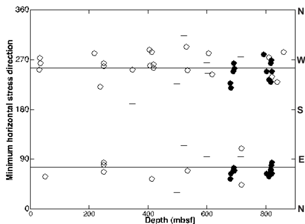
Fig. 2 - Estimates of minimum stress direction (excluding possible natural fractures) vs. depth. Symbols: breakouts (solid dots), petal centre-line and core-edge (open circles), and tensile cracks (-). Horizontal lines indicate mean orientation of minimum stress ( 75^\circ and 255^\circ , or N75^\circ E and S75^\circ W ).
