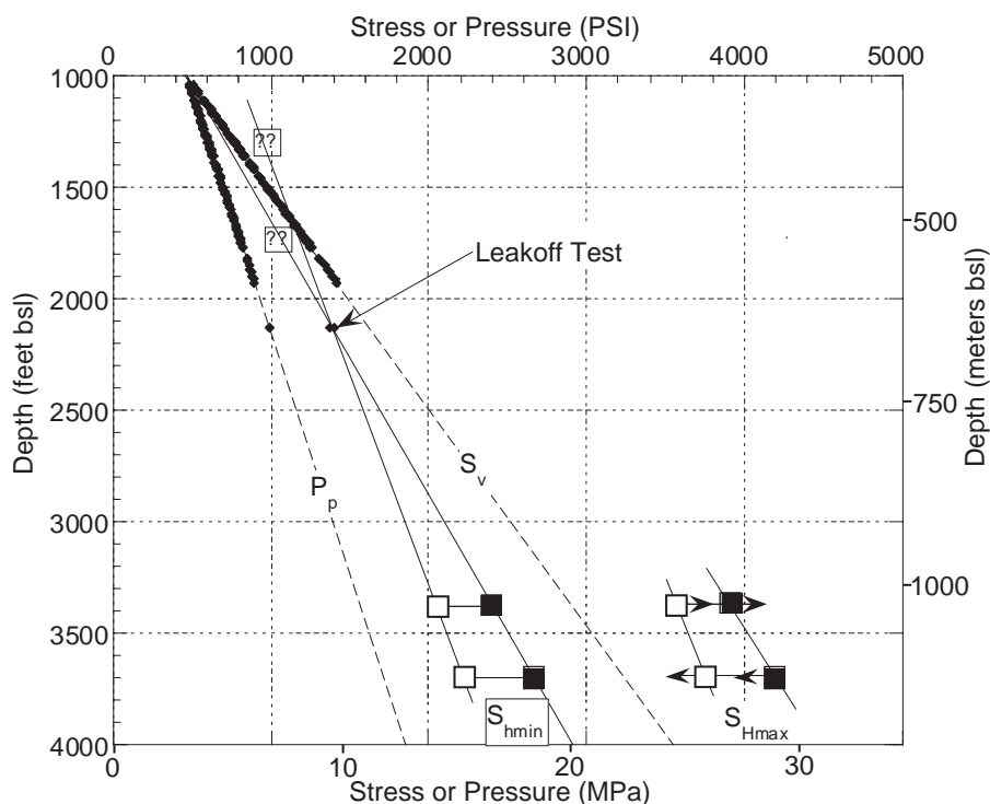
Fig. 4 - Stress analysis results. S_v is computed from integration of laboratory measurements. P_p is computed assuming a gradient of 0.465 psi/ft (0.001 MPa/m). The two lines for S_{hmin} are (a) assuming that it is equal to S_v at the sea floor, and (b) assuming that it has a finite value at the sea floor. Both assumptions are reasonable, but a finite value is more likely. S_{hmax} values are constrained by the following: (1) observations of tensile cracks at 1010 m bsl (where excess pumping may have contributed to their formation) and no tensile fractures at immediately below that depth and at approximately 1105 m bsl, and (2) the assumed projection of the S_{hmin} gradient to those depths.
