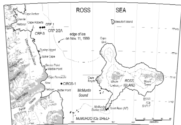
Fig. 1 - Map of the south west corner of the Ross Sea, showing the locations of the CRP-1, CRP-2/2a, and CRP-3 drill sites (Taken from Cape Roberts Science Team, 2000).
