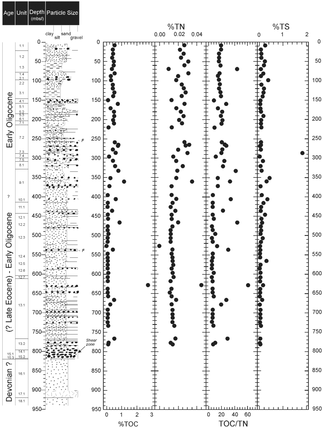
Fig. 2 - Comparison of values of TOC, TN, TS and TOC:TN with the lithology of CRP-3 core (Cape Roberts Science Team, 2000; p. 7).
