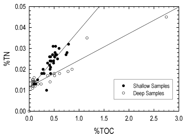
Fig. 4 - Plot of TN versus TOC for CRP-3 samples. Lines are the result of least squares regressions of the shallow (depth < 330 mbsf) and deep (depth > 330 mbsf) samples.
