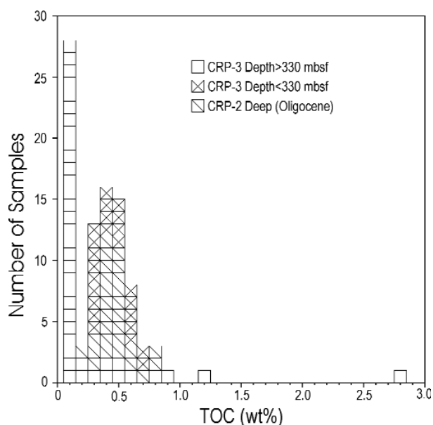
Fig. 3 - Comparison of TOC values in CRP-3 samples obtained from above 330 mbsf, below 330 mbsf and with the Oligocene section in CRP-2/2A.
