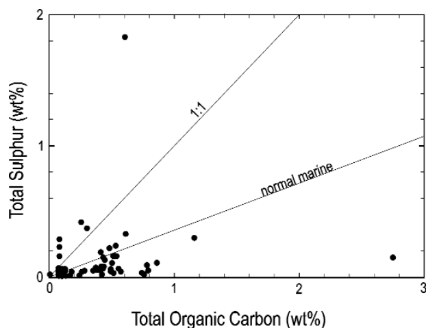
Fig. 5 - Plot of TS versus TOC for CRP-3 samples with "normal marine" trends and unit TS:TOC ratio shown for reference.
