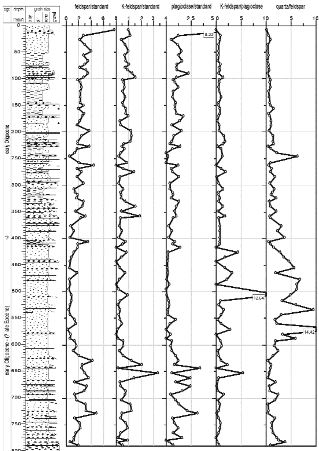
Fig. 3 - Abundance of total feldspar, K-feldspar and plagioclase, K-feldspar/plagioclase ratio and quartz/feldspar ratio in the Cenozoic CRP-3 sediments. Lithology simplified after Cape Roberts Science Team (2000).
