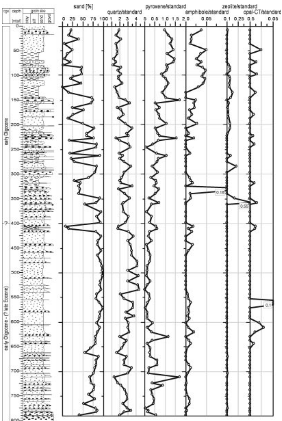
Fig. 2 - Sand content (63 \mu\text{m} - 2 mm), abundance of quartz, pyroxene, amphibole, zeolite and opal-CT in the Cenozoic CRP-3 sediments. Lithology simplified after Cape Roberts Science Team (2000).
