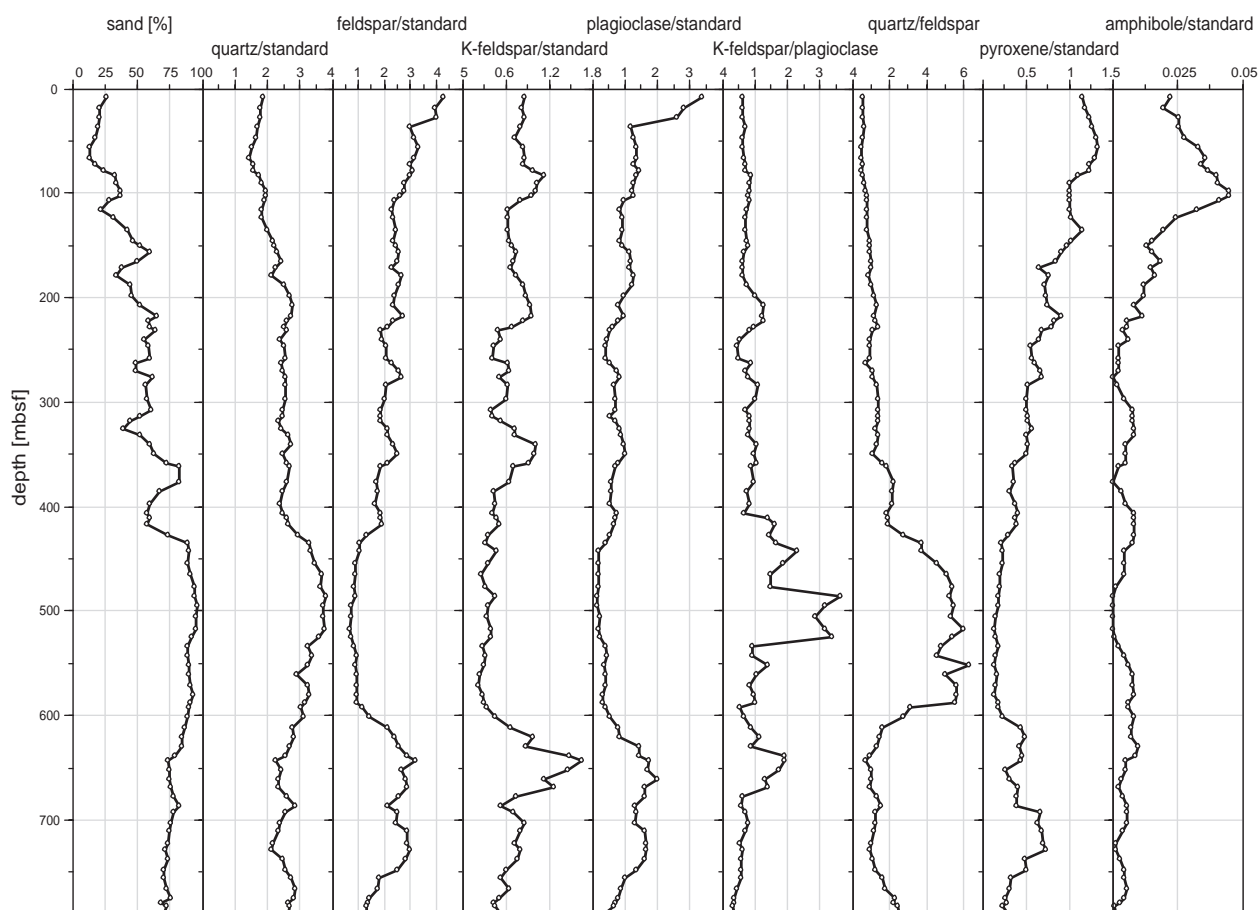
Fig. 4 - Smoothed (5-point-average) abundance of bulk mineralogy in the Cenozoic CRP-3 sediments (The outliers in quartz/feldspar at 246.03 mbsf and in amphibole/standard at 330.97 mbsf had been removed prior to the calculations).
