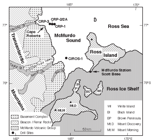
Fig. 1 - Location of the drillsites CRP-1, CRP-2/2A and CRP-3 on the continental shelf of McMurdo Sound in Ross Sea, Antarctica, and generalised geology of the hinterland (after Warren, 1969).
