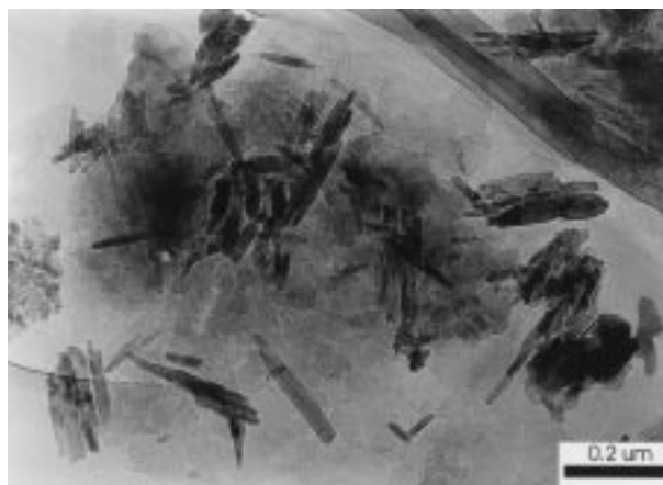
Fig. 12 - Core level 918.53 mbsf, TEM image showing aluminous smectites and kaolinites.
