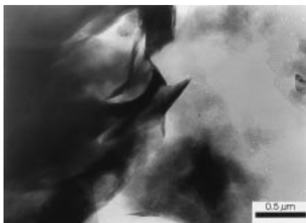
Fig. 7 - Core level 680.65 mbsf, TEM image showing detail of curled edge of authigenic Mg-smectite particle.
