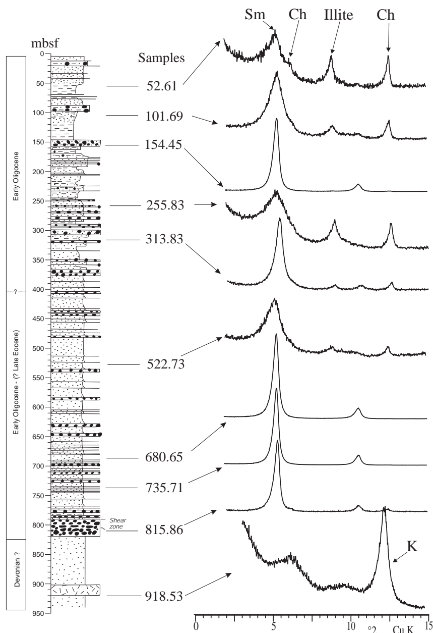
Fig. 1 - Lithostratigraphic column of the CRP-3 core with some typical XRD patterns (glycolated samples) of the clay fraction of the sediments. Sm = Smectite, Ch = Chlorite, K = Kaolinite
