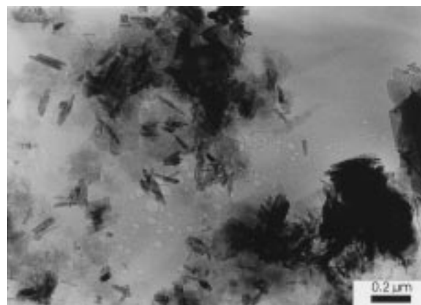
Fig. 11 - Core level 919.06 mbsf, TEM image showing aluminous smectites and Fe-oxydes.
