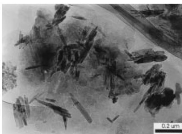
Fig. 9 - Core level 901.2 mbsf, TEM image showing smectite and Fe-oxides.
