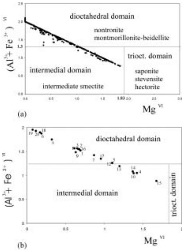
Fig. 2 - a) Octahedral composition of individual smectite particles: (Al 3+ +Fe 3+ ) VI vs. Mg VI , the compositional fields of dioctahedral, intermediate and trioctahedral domains from the literature (see text); b) plots of average chemical composition of smectites from each level.
