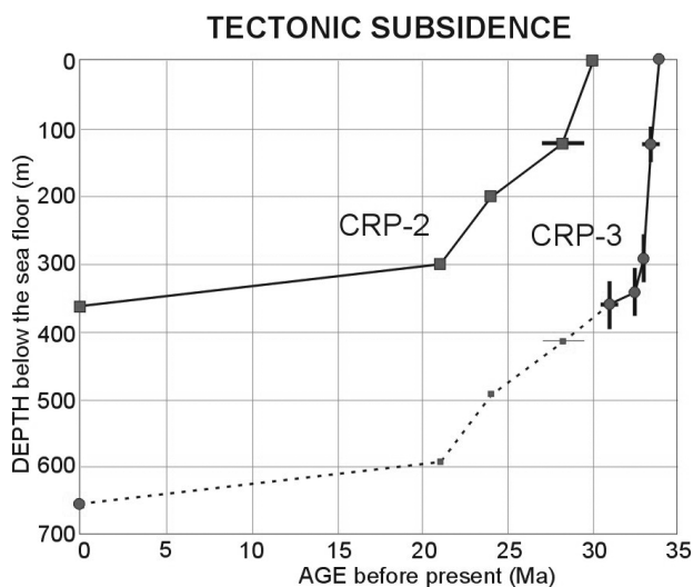
Fig. 1 - Tectonic subsidence curves obtained using backstripping technique at the CRP-2 (squares) and the CRP-3 (circles) drillsites. The dashed curve represents the extrapolated tectonic subsidence of the basement at CRP-3 site between 31 Ma and present. This curve is inferred from the trend at CRP-2 (from 30 to 21 Ma) and the depth of the basement caused by the tectonics at present time at the CRP-3 site. The error bars indicate the range of the uncertainties in the palaeo-depth information and age.
