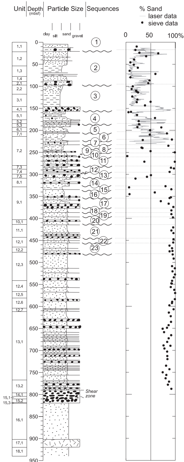
Fig. 1 - Lithologic log for the CRP-3 core, showing unit and sequence boundaries, and variations in percent sand from sieve-Sedigraph analyses. Comparative data for percent sand determined from small (>1 g) samples by Malvern (laser) size analysis (Fielding, Dunbar & Bryce, this volume).
