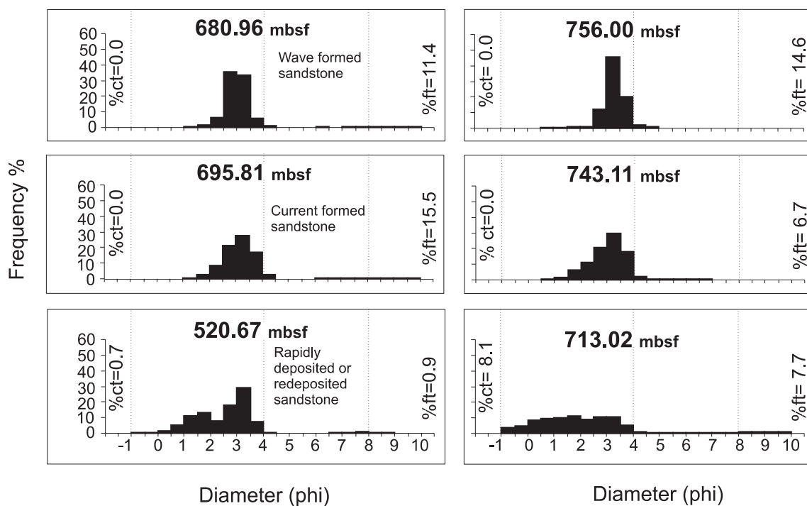
Fig. 3 - Histograms of sandstone samples from the older sand-dominated section of CRP-3, showing typical examples of sand modes interpreted as wave-formed (bell-shaped, narrow), current-formed (bell-shaped, broader) and rapidly deposited (broad, rectangular or bimodal). All but one of the six samples have virtually no silt, but between 7 and 16% clay, which is most likely to have been precipitated after deposition.
