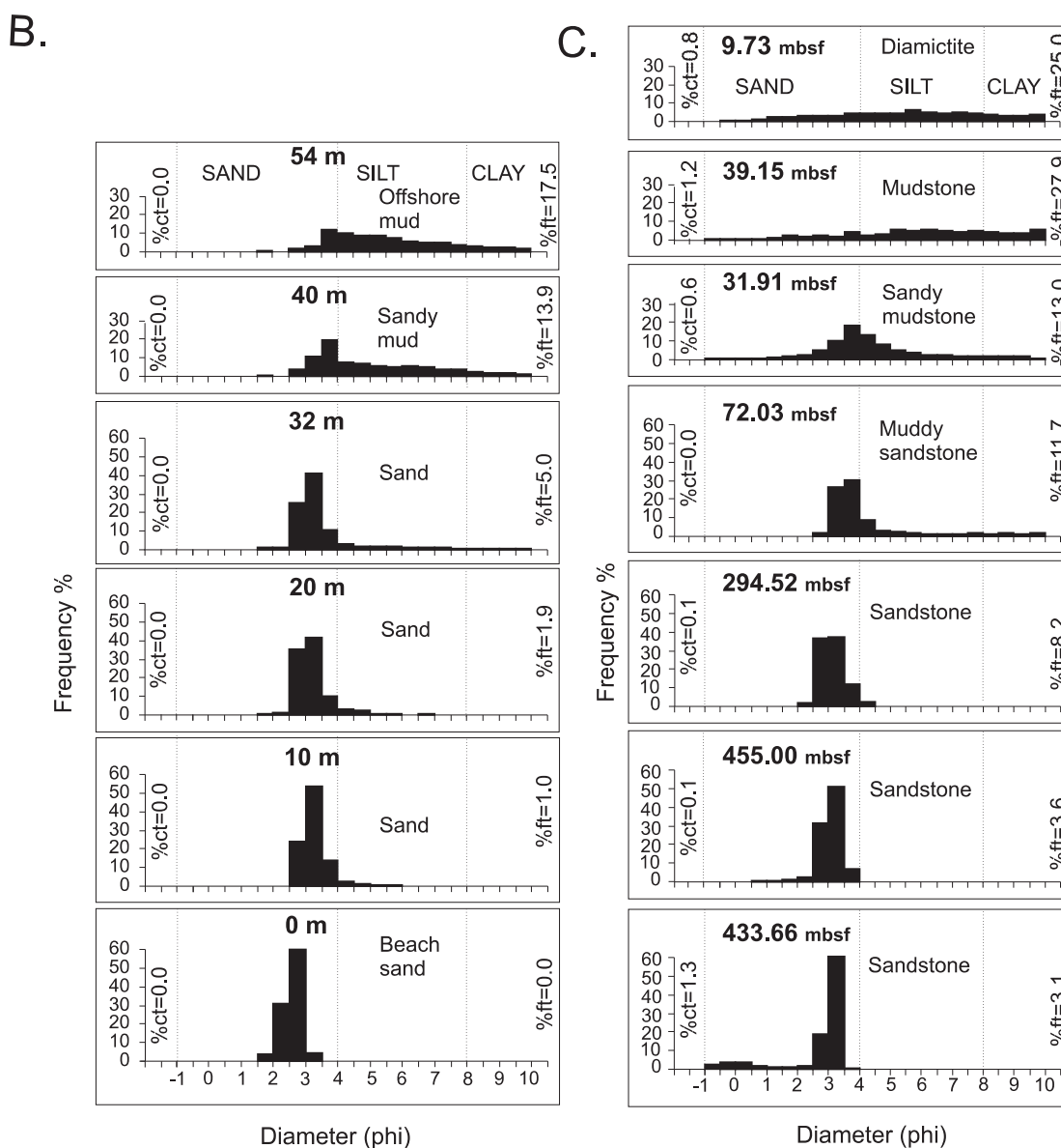
Fig. 2 - Facies model for coastal sedimentation, accompanied by textural data from a transect off a present day wave-dominated coast, and from a selection of CRP-3 samples. A. Model for wave-dominated nearshore coastal sedimentation (from Barrett, 1989, adapted from Elliott, 1986). B. Histograms of modern sea floor sediment from a transect from offshore mud to beach sand off PekaPeka, 50 km north of Wellington, NZ, showing the progressive onshore increase in sand content and improved sorting of the sand mode. Water depth for each sample shown with histogram in m. C. Histograms of CRP-3 samples chosen for illustrative comparison with the sediment accumulating off Peka Peka. Note, however, the coarse tail of coarse sand in samples from 31.91, 39.15, 298 and 433 mbsf, interpreted as ice-rafted debris.
