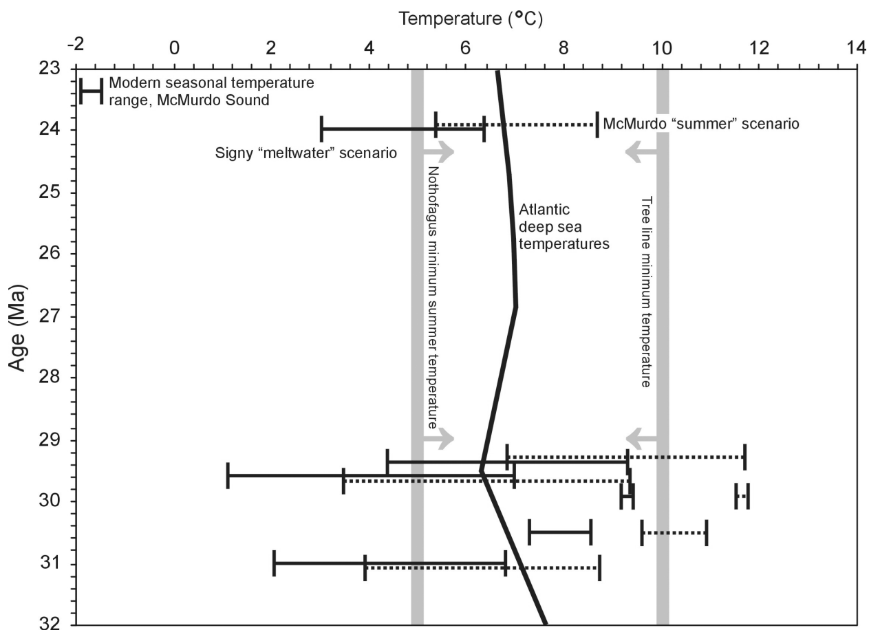
Fig. 2 - Marine palaeotemperature estimates vs. depositional age for shelf waters in the McMurdo Sound region during the early Oligocene and earliest Miocene. Atlantic deep sea temperatures are from Lear et al. (2000).
