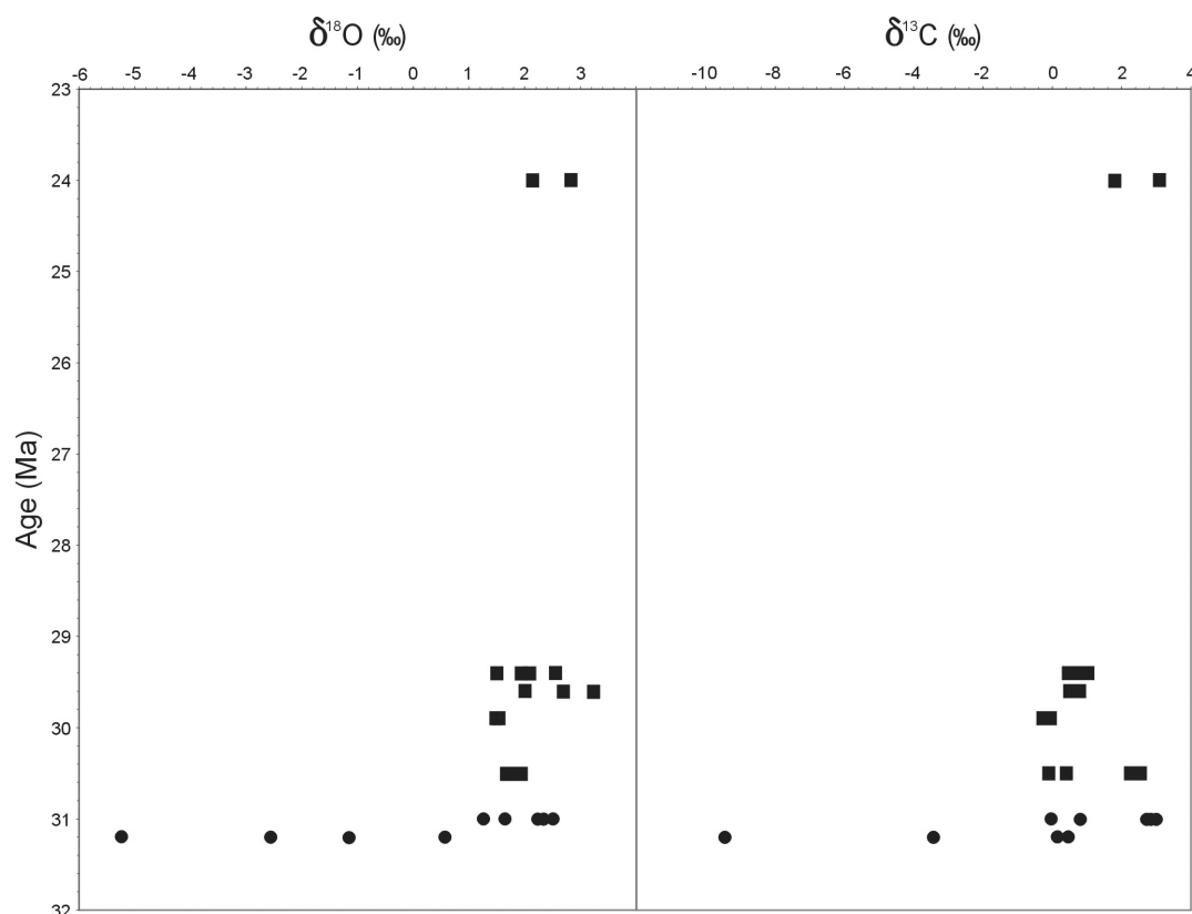
Fig. 1 - \delta^{18}\text{O} and \delta^{13}\text{C} data vs. depositional age for CRP-2/2A and CRP-3 drillholes. Filled squares = aragonite shells; filled circles = calcite shells. Measurement errors fall within the symbols.
