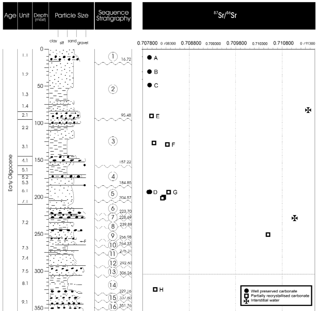
Fig. 2 - Strontium isotope results from well-preserved bivalve fragments, recrystallised bivalve and echinoid fragments, and interstitial waters for the upper 350 mbsf of CRP-3. 2SE error bars fall within the individual symbols. Also shown are lithological units, a simplified sedimentary log and sequence stratigraphy. Sequence boundaries are annotated with their exact depths (mbsf).
