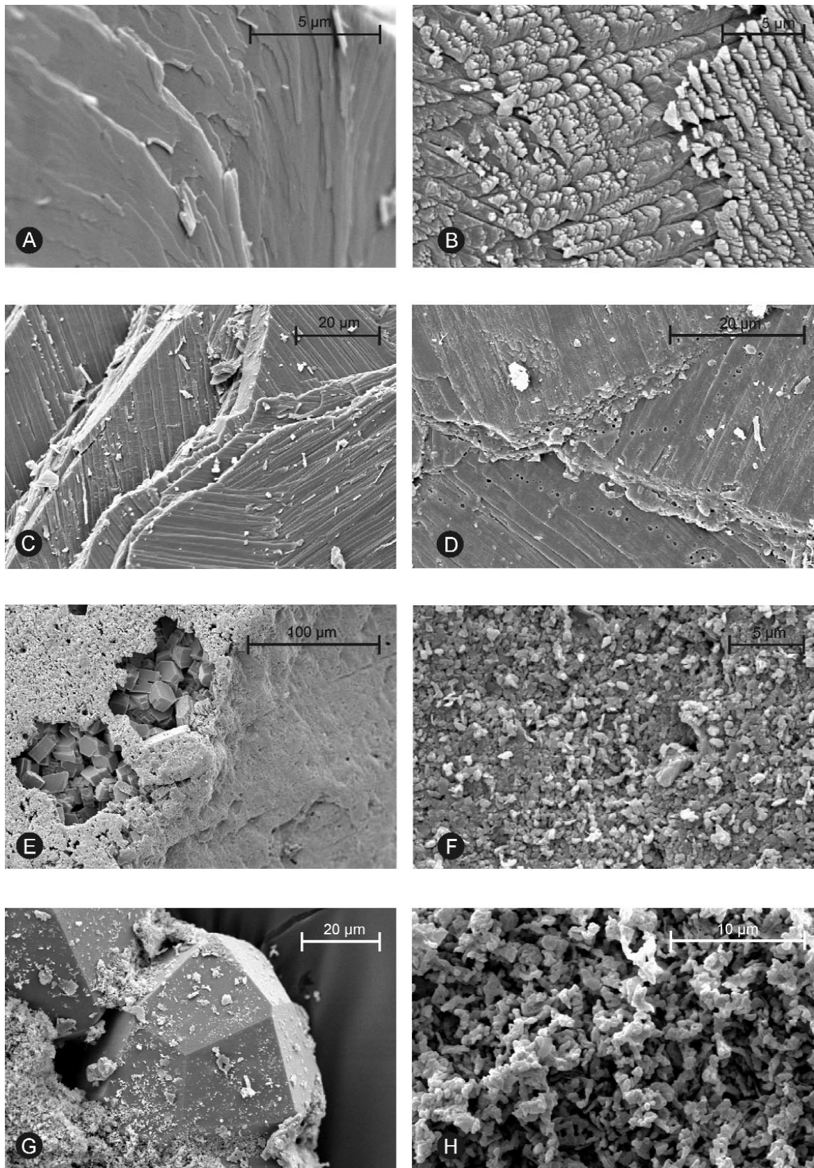
Fig. 1 - Scanning electron micrographs of preserved ultrastructures from selected representative CRP-3 carbonate samples: A) 10.88 mbsf, horizontal section through well-preserved aragonitic modiolid bivalve. B) 29.94 mbsf, oblique section through well-preserved pectinid bivalve fragment displaying three first-order lamellae of crossed foliated calcite. C) 47.55 mbsf, horizontal section through well-preserved pectinid bivalve displaying four first-order lamellae of crossed foliated calcite. D) 190.29 mbsf, horizontal section through well preserved pectinid bivalve displaying three first-order lamellae of crossed foliated calcite. E) 89.02 mbsf, poorly preserved unidentified bivalve showing localised sparry calcite precipitation overlying original aragonite. F) 127.48 mbsf, horizontal section through poorly preserved unidentified bivalve displaying fine-grained amorphous calcite texture. G) 190.50 mbsf, close-up view of calcite overgrowth on unidentified bivalve. H) 320.36 mbsf, close up view of coarse-grained amorphous calcite from poorly preserved unidentified bivalve.
