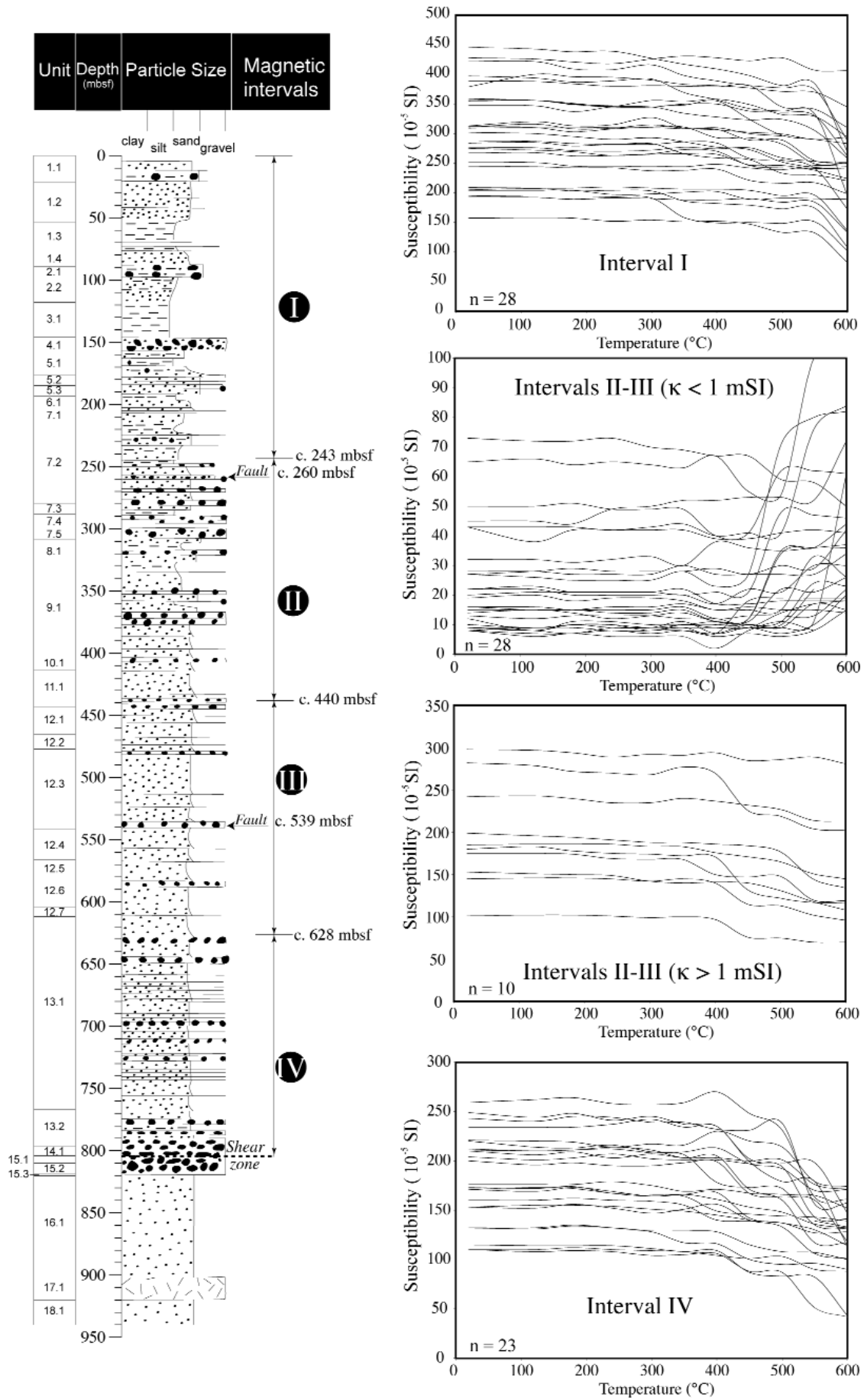
Fig. 2 - Changes in the low-field magnetic susceptibility ( \kappa ) during thermal demagnetization for pilot samples from different stratigraphic intervals in CRP-3.
